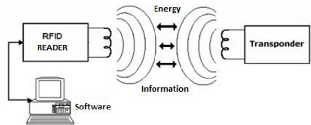
Figure 1: Diagram of a RFID system.
