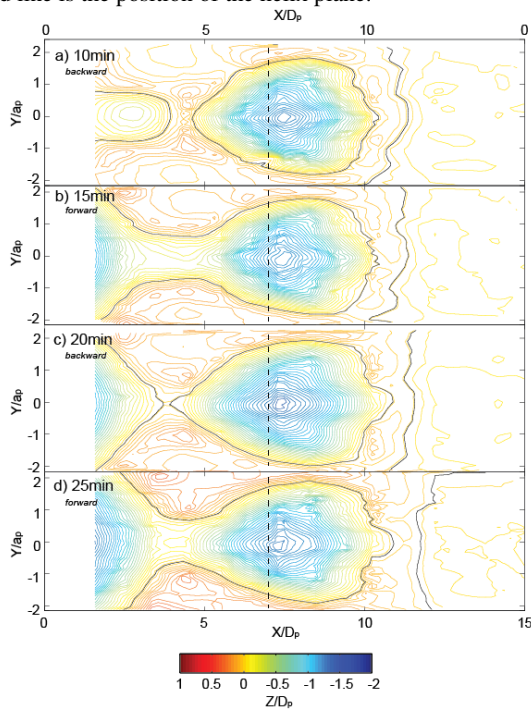
Figure 12: Contour plot evolution of the back and forth scenario with a speed revolution of 400 rpm using the bow-thrusters configuration. Dashed line is the position of the helix plane.
