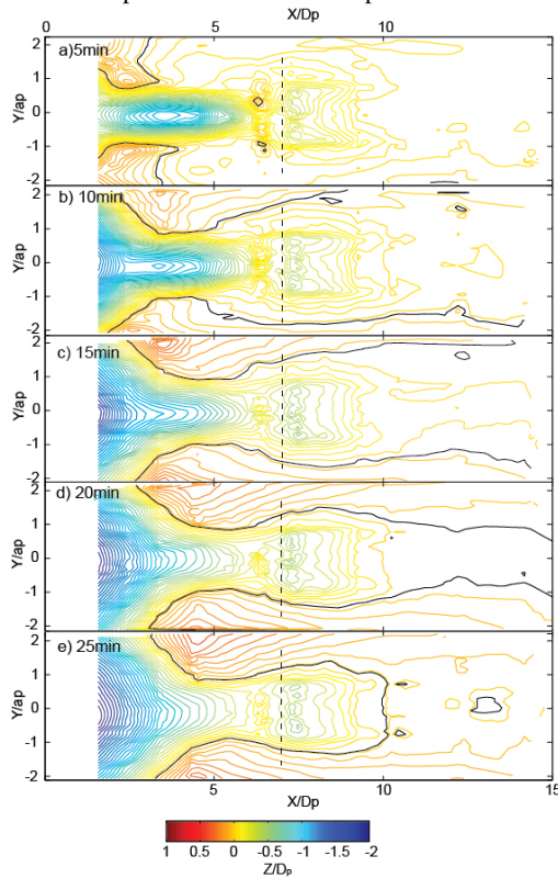
Figure 9: Contour plot evolution of bow-thrusters scenario, with a speed revolution of 400rpm. Dashed line is the position of the helix plane.
