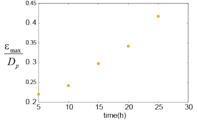
Figure 10: Maximum scouring depth evolution for the bow-thrusters scenario with a speed revolution of 400rpm.
