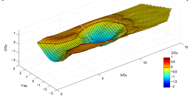
Figure 11: Scour due to bow-thruster after 15 min forward at 400 rpm
