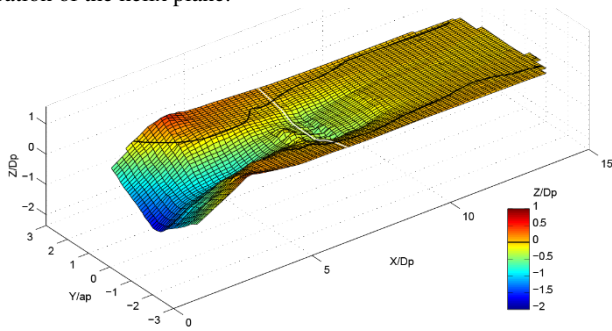
Figure 8: Rendering of the scour action produced by twin bow thrusters moving forward after 15 minutes run at 400 rpm. White line is the location of the helix plane.
