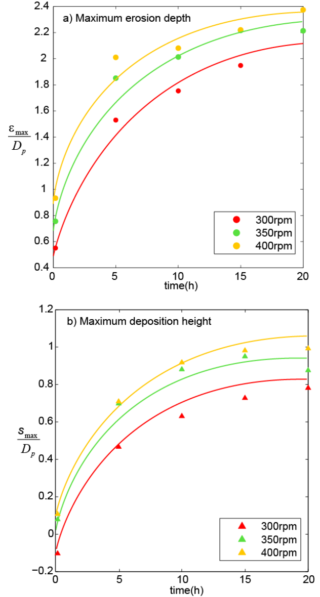
Figure 7: Evolution of the a) maximum scouring depth and b) maximum deposition height
