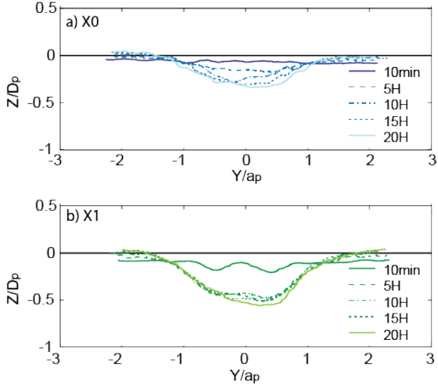
Figure 6: Transversal profiles in the X0 and X1 location, scanned for the 300 rpm scenario.
