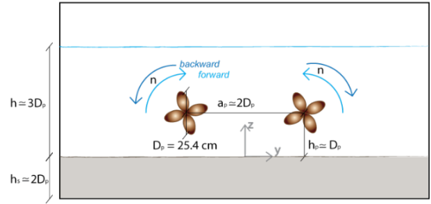
Figure 2: Sketch of the thruster system
