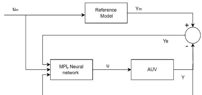
Figure 5: Block diagram of MRAC combined with MLP NN.
