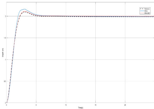
Figure 6: Depth control with classic MRAC and MRACMLP.
