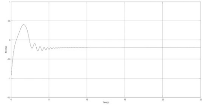
Figure 7: Control output with classic MRAC.
