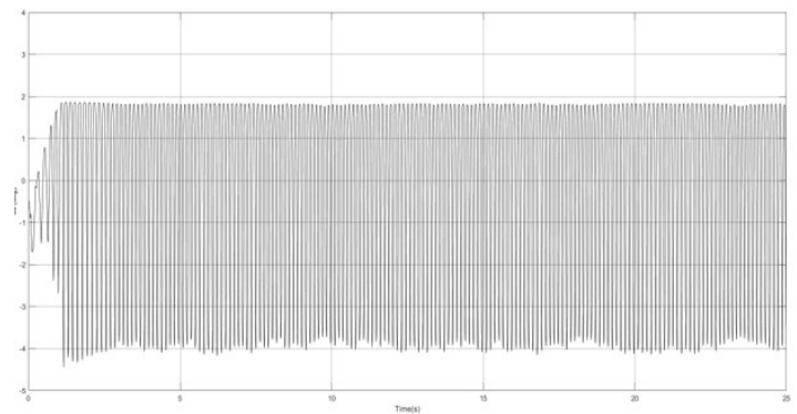
Figure 14: Control output with MRAC combined with MLP NN with uncertainties.
