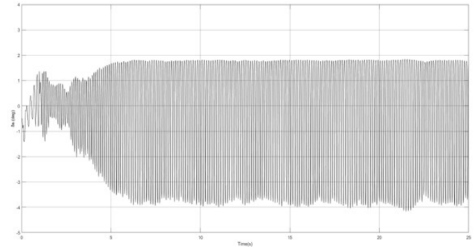
Figure 8: Control output with MRAC combined with MLP NN.
