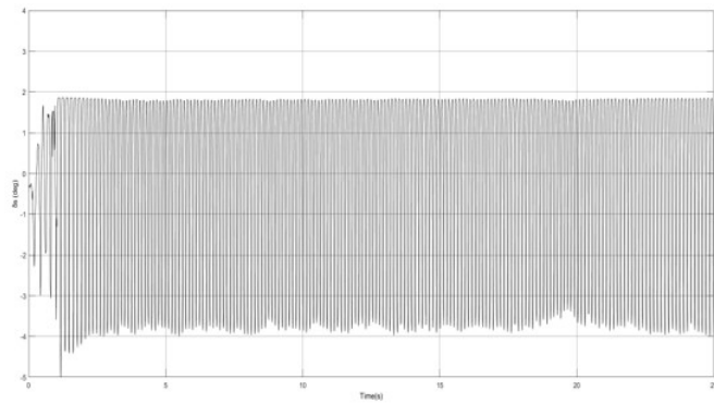
Figure 11: Control output with MRAC combined with MLPNN in noise presence.
