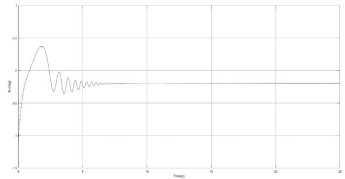
Figure 13: Control output with classic MRAC with uncertainties.
