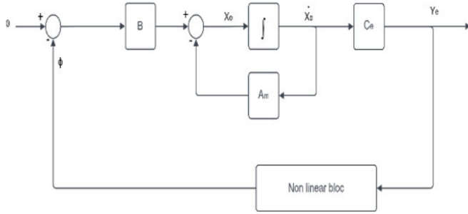
Figure 3: Closed-loop of hyper-stable system.
