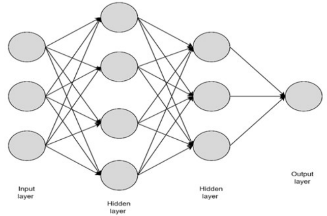
Figure 4: MLP neural network structure.
