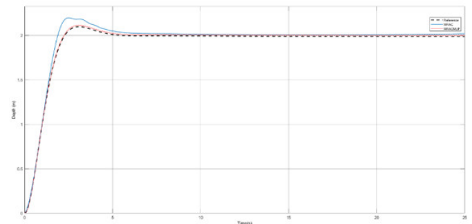
Figure 9: Depth control with classic MRAC and MRACMLP in noise presence.
