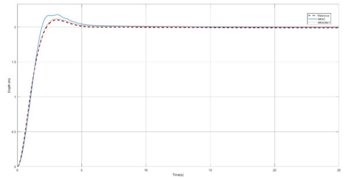
Figure 12: Depth control with classic MRAC and MRACMLP- With uncertainties.
