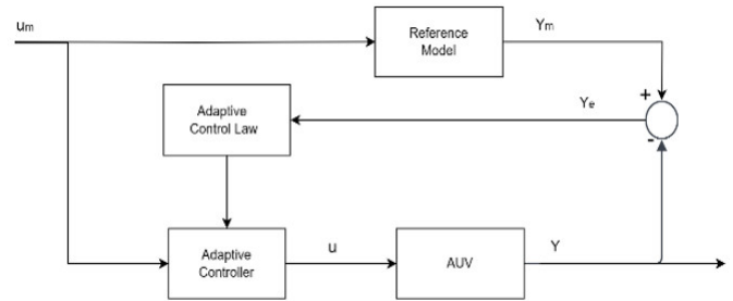
Figure 2: Structure of direct MRAC for an AUV.
