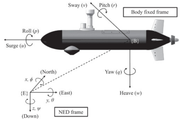
Figure 1: General AUV Structure with Reference Frame.
